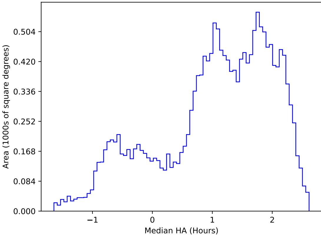
weather_cloudso14v3.4_10yrs WFD z band: Median HA
