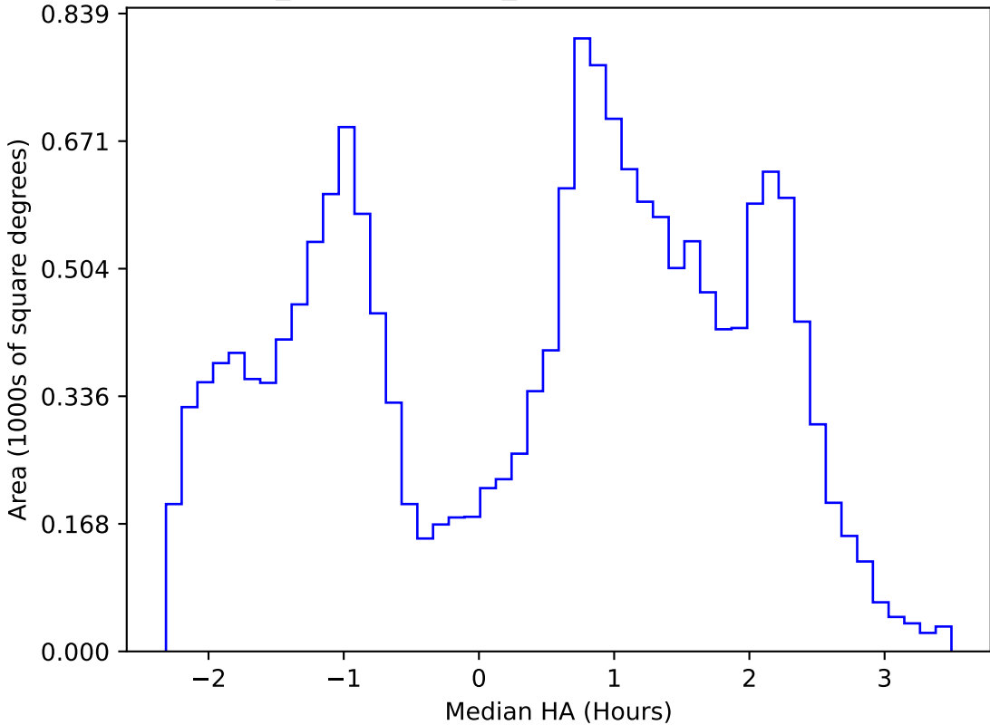
weather_cloudso14v3.4_10yrs WFD u band: Median HA
