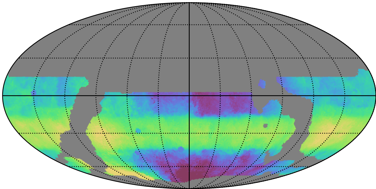
weather_cloudso14v3.4_10yrs WFD i band: Median HA
