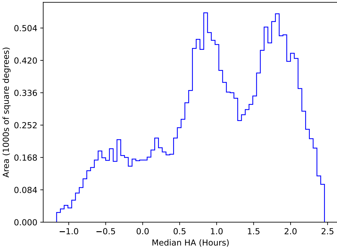
weather_cloudso14v3.4_10yrs WFD i band: Median HA
