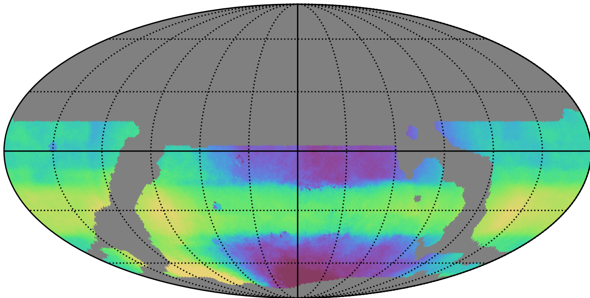
weather_cloudso14v3.4_10yrs WFD all bands: Median HA
