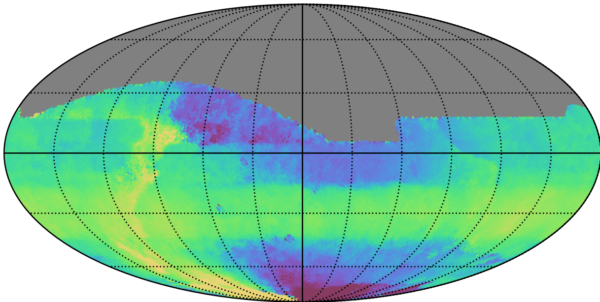
weather_cloudso14v3.4_10yrs All sky z band: Median HA
