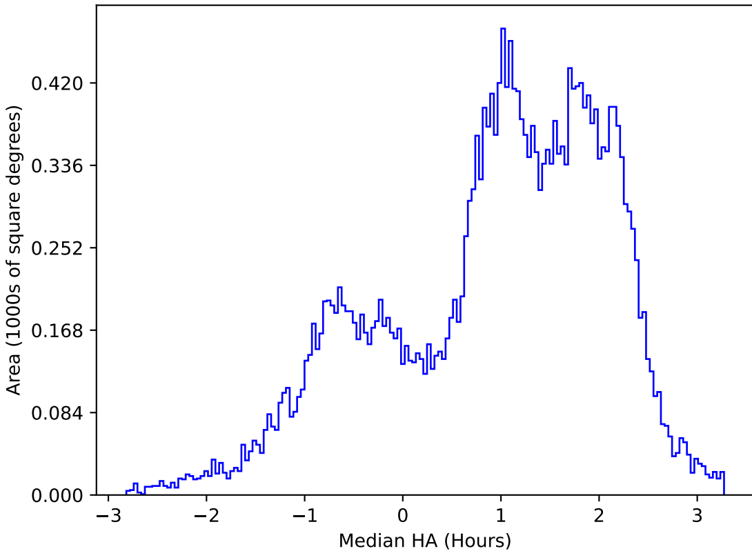
weather_cloudso14v3.4_10yrs All sky z band: Median HA
