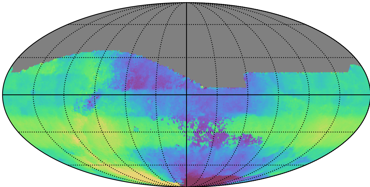
weather_cloudso14v3.4_10yrs All sky r band: Median HA
