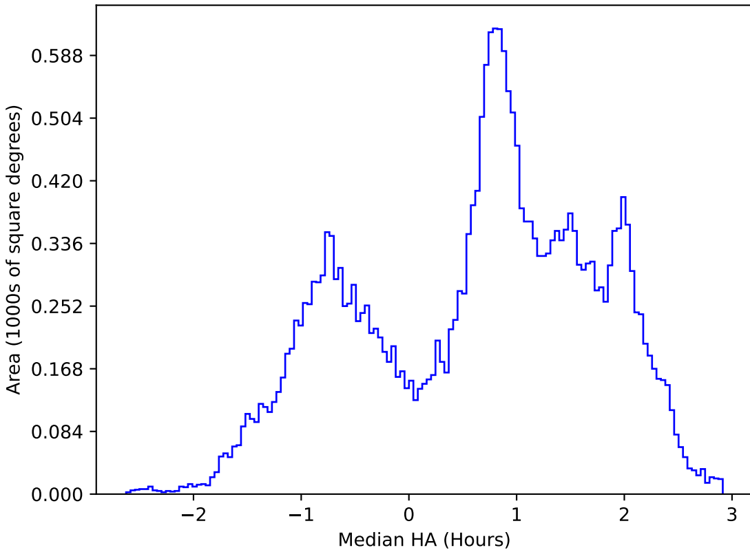
weather_cloudso14v3.4_10yrs All sky r band: Median HA
