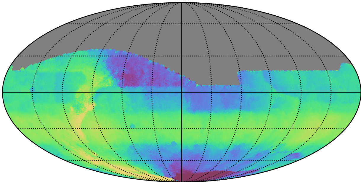
weather_cloudso14v3.4_10yrs All sky i band: Median HA
