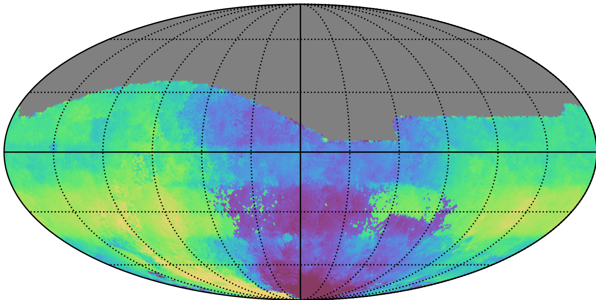
weather_cloudso14v3.4_10yrs All sky g band: Median HA
