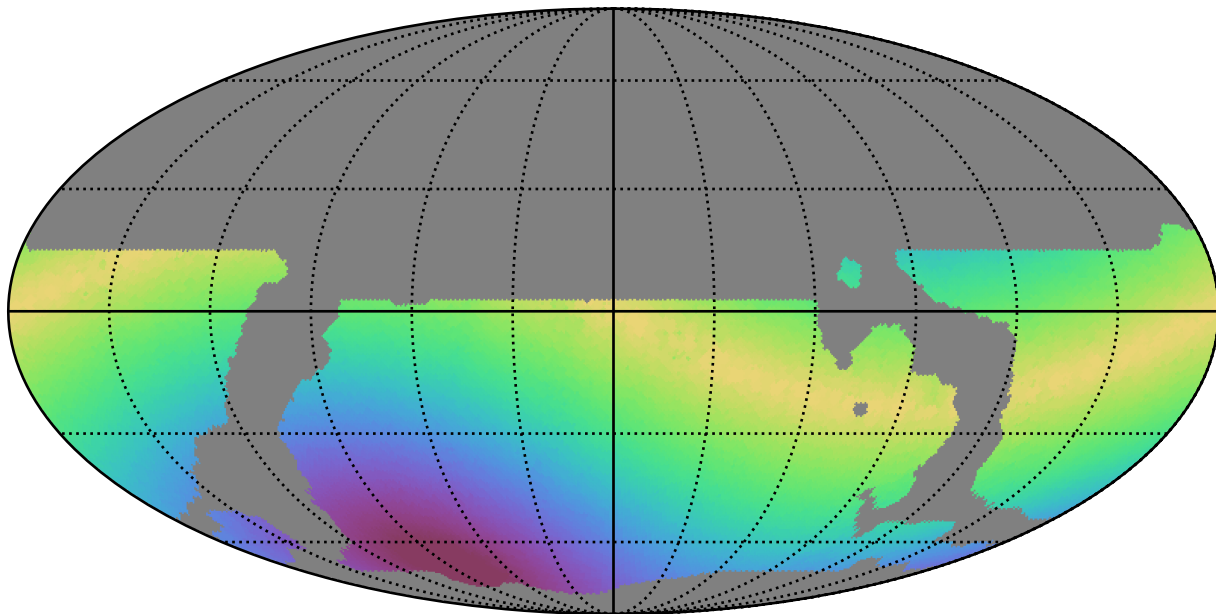
weather_cloudso14v3.4_10yrs WFD u band: Max solarElong
