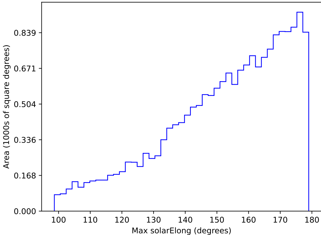
weather_cloudso14v3.4_10yrs WFD u band: Max solarElong
