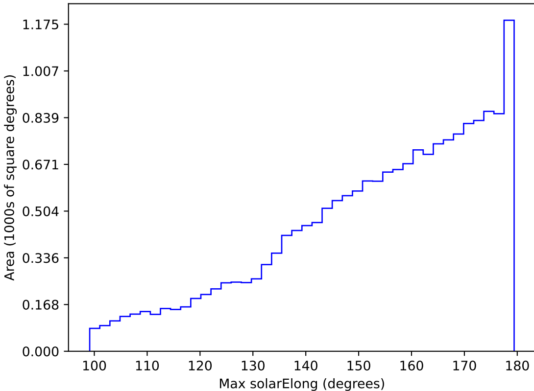
weather_cloudso14v3.4_10yrs WFD r band: Max solarElong
