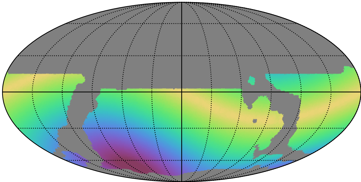
weather_cloudso14v3.4_10yrs WFD all bands: Max solarElong
