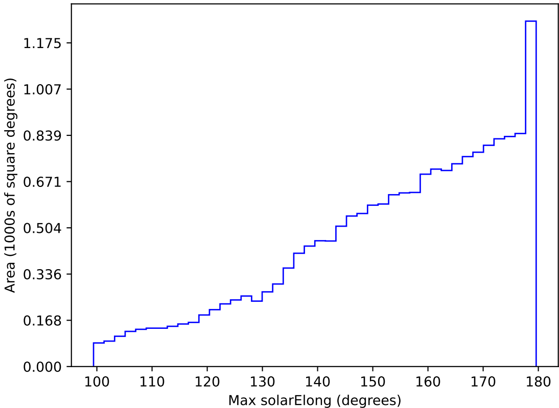
weather_cloudso14v3.4_10yrs WFD all bands: Max solarElong
