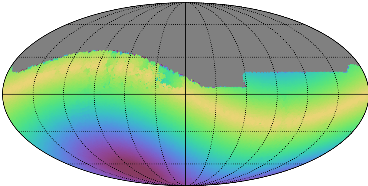
weather_cloudso14v3.4_10yrs All sky z band: Max solarElong
