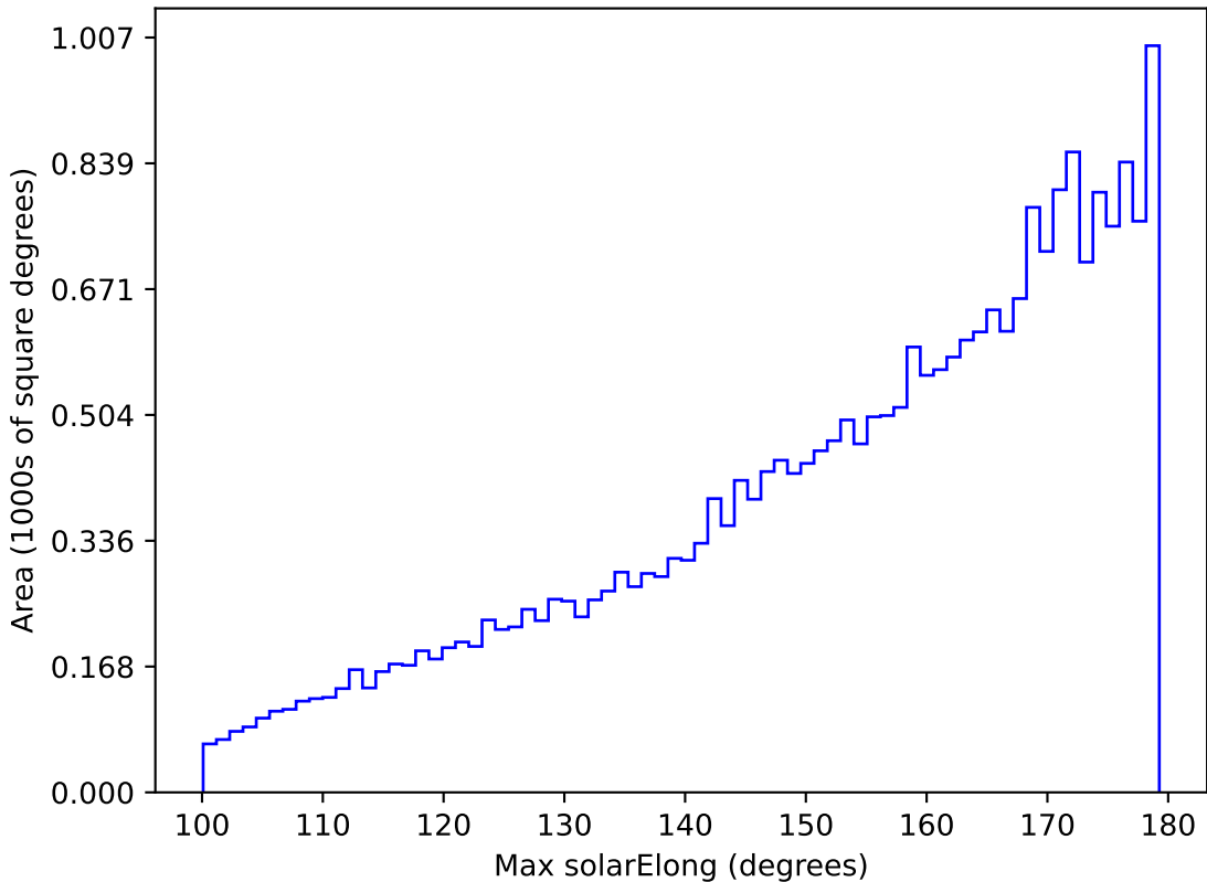
weather_cloudso14v3.4_10yrs All sky z band: Max solarElong
