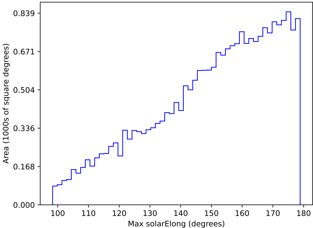
weather_cloudso14v3.4_10yrs All sky u band: Max solarElong
