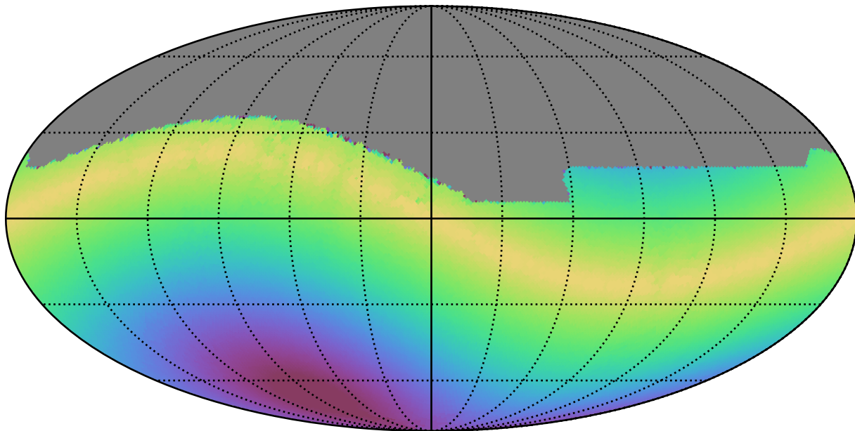
weather_cloudso14v3.4_10yrs All sky r band: Max solarElong
