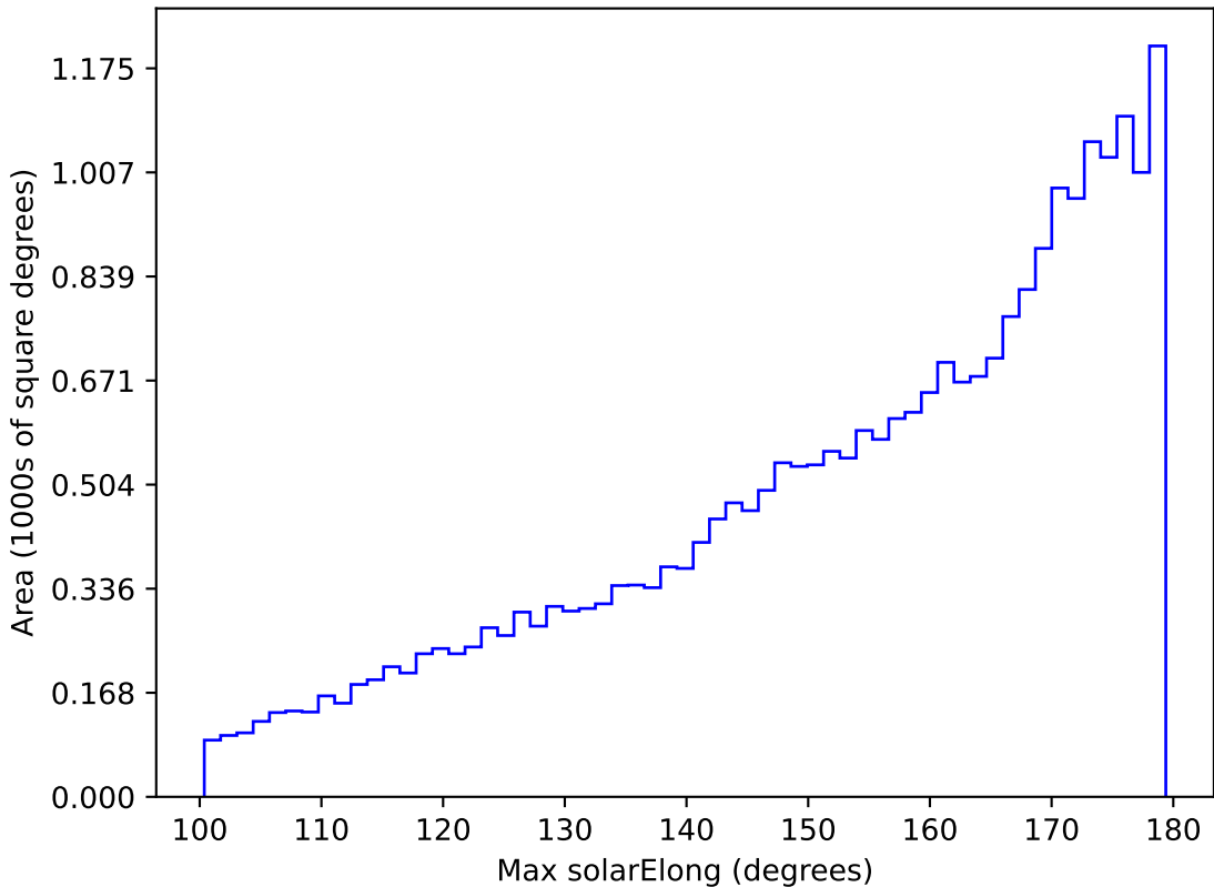
weather_cloudso14v3.4_10yrs All sky r band: Max solarElong
