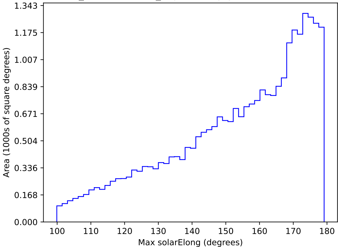
weather_cloudso14v3.4_10yrs All sky g band: Max solarElong
