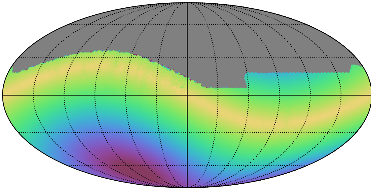
weather_cloudso14v3.4_10yrs All sky all bands: Max solarElong
