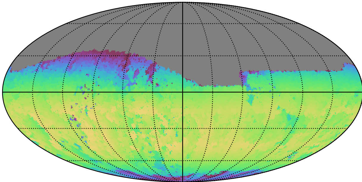
weather_cloudso14v3.4_10yrs Yr 1 z band: Max skyBrightness
