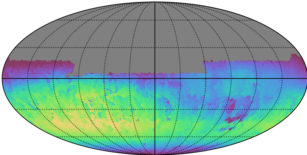
weather_cloudso14v3.4_10yrs Yr 1 u band: Max skyBrightness
