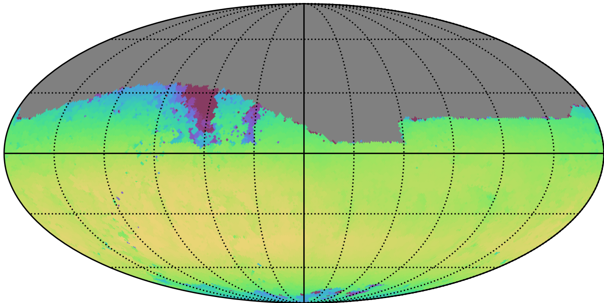
weather_cloudso14v3.4_10yrs Yr 1 i band: Max skyBrightness
