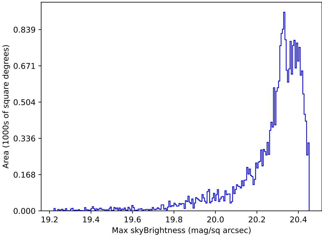
weather_cloudso14v3.4_10yrs Yr 1 i band: Max skyBrightness
