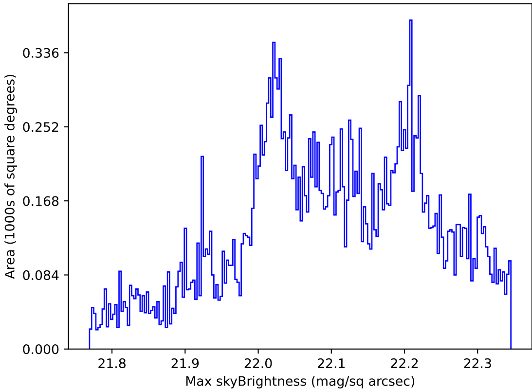
weather_cloudso14v3.4_10yrs Yr 1 g band: Max skyBrightness
