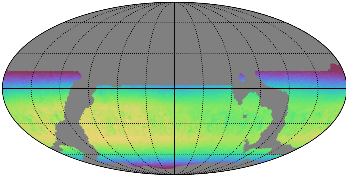
weather_cloudso14v3.4_10yrs WFD z band: Max skyBrightness
