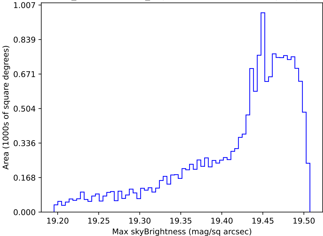
weather_cloudso14v3.4_10yrs WFD z band: Max skyBrightness
