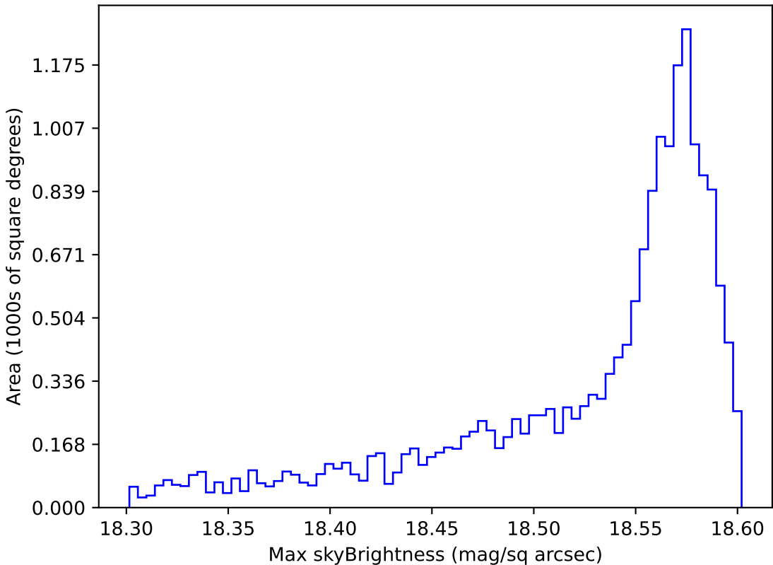
weather_cloudso14v3.4_10yrs WFD y band: Max skyBrightness
