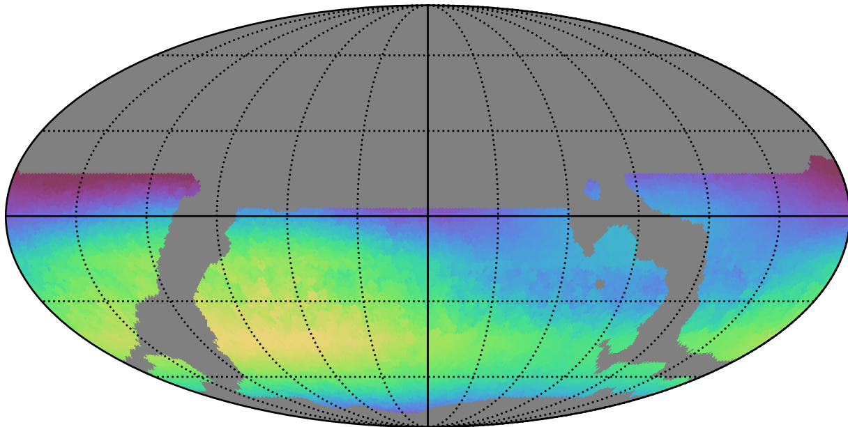
weather_cloudso14v3.4_10yrs WFD u band: Max skyBrightness
