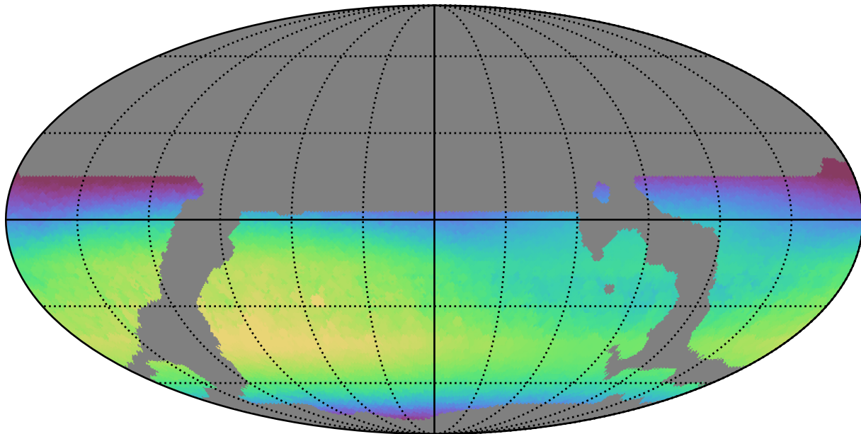
weather_cloudso14v3.4_10yrs WFD i band: Max skyBrightness
