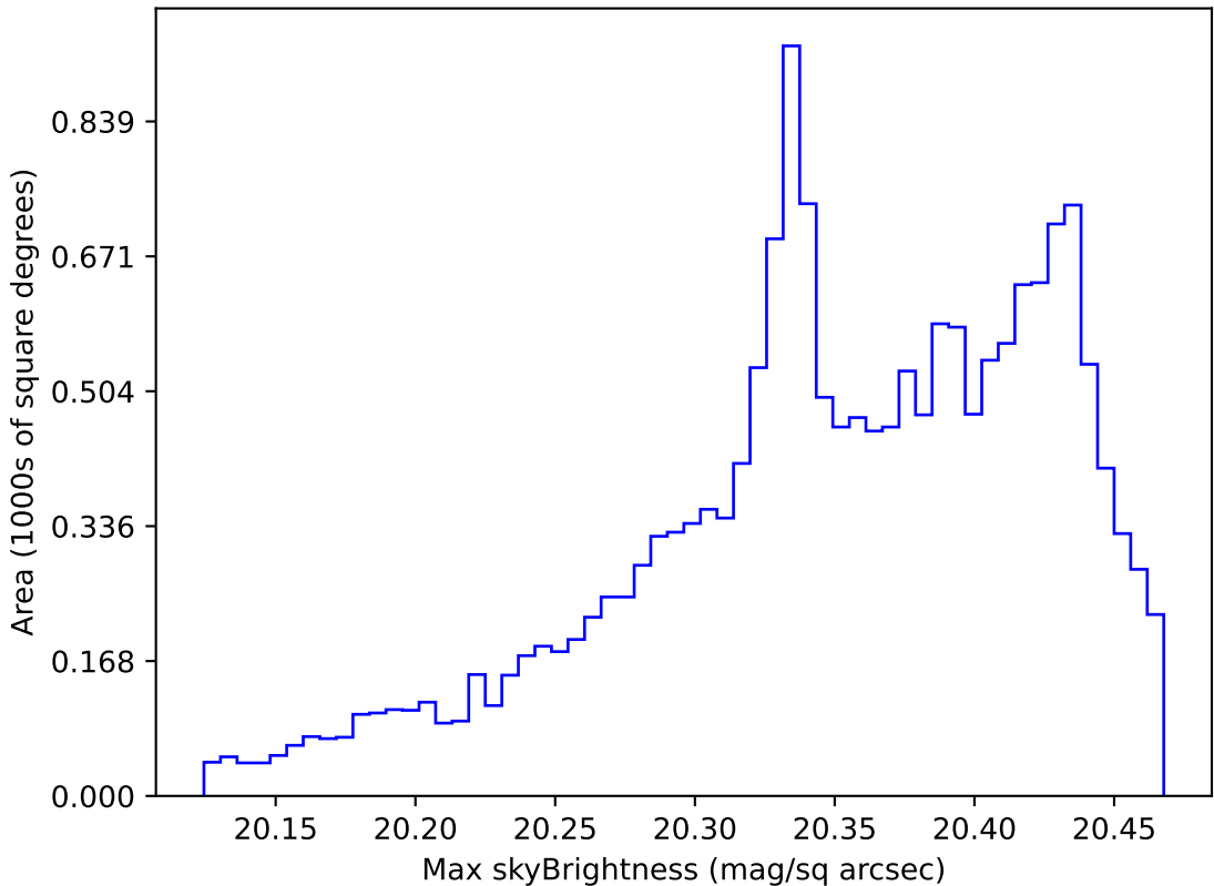
weather_cloudso14v3.4_10yrs WFD i band: Max skyBrightness
