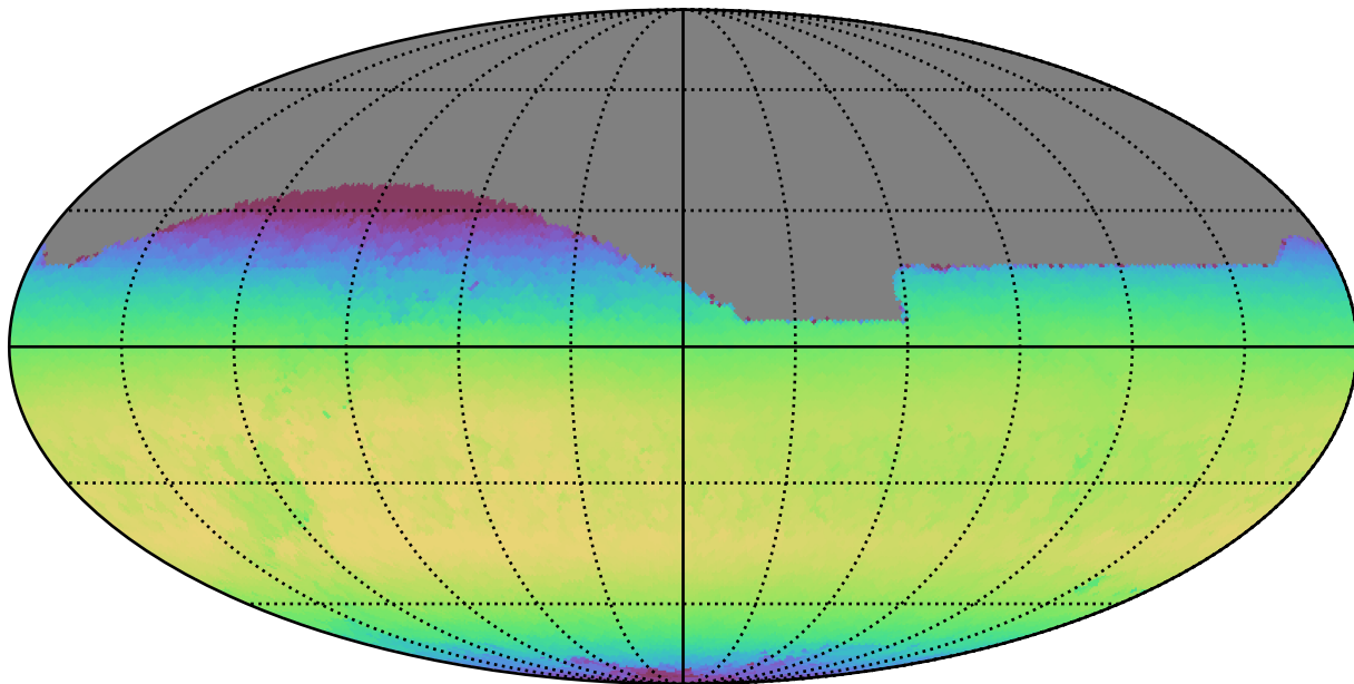
weather_cloudso14v3.4_10yrs All sky z band: Max skyBrightness
