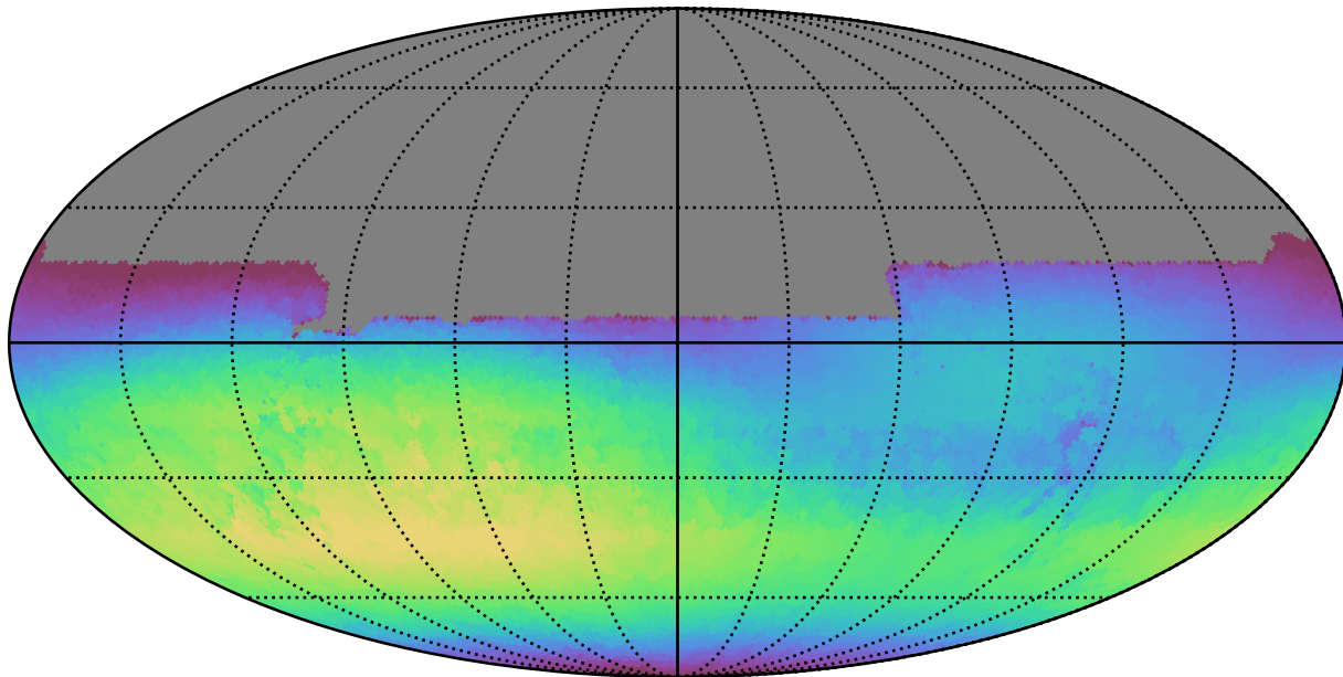
weather_cloudso14v3.4_10yrs All sky u band: Max skyBrightness
