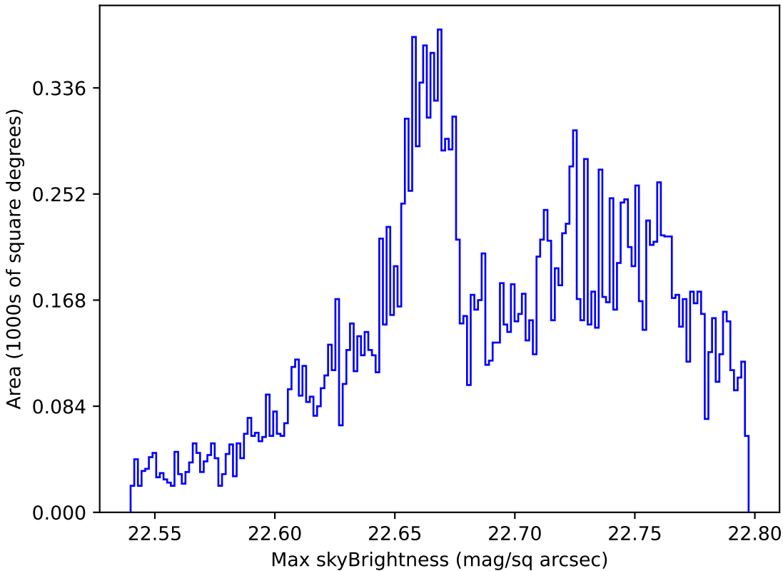
weather_cloudso14v3.4_10yrs All sky u band: Max skyBrightness
