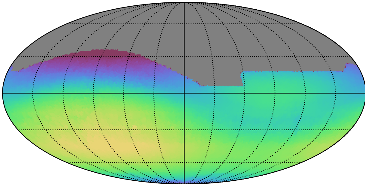
weather_cloudso14v3.4_10yrs All sky r band: Max skyBrightness
