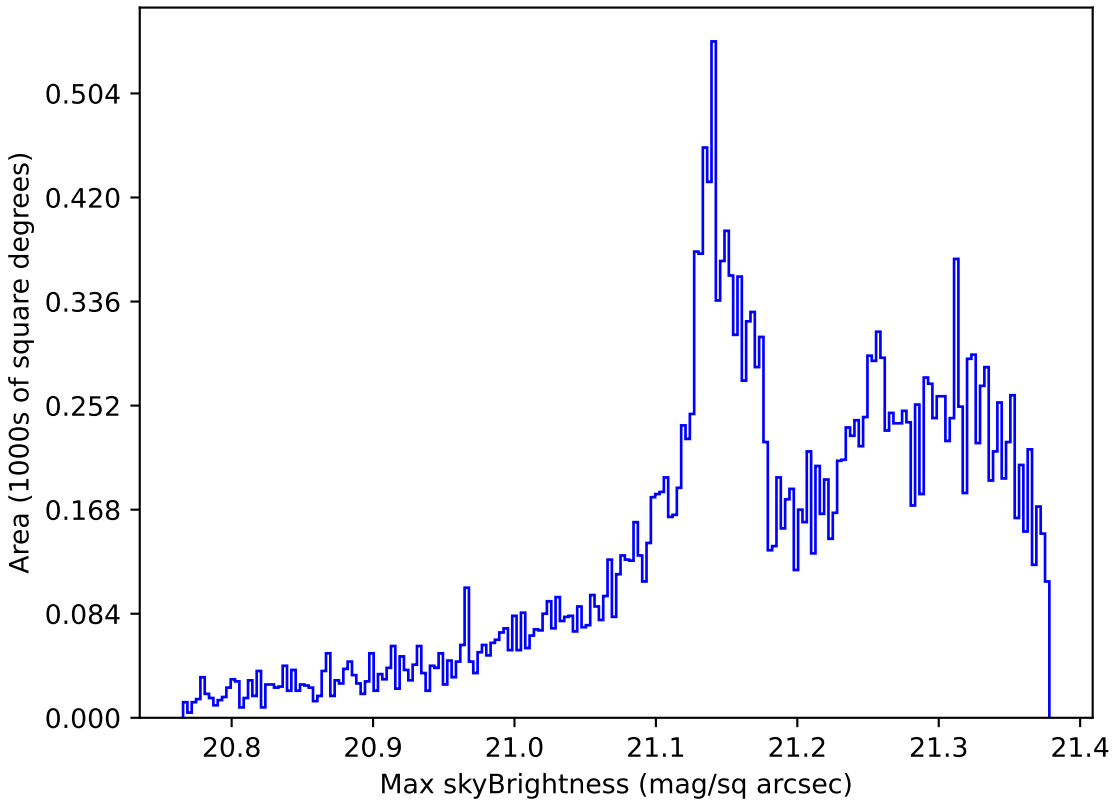
weather_cloudso14v3.4_10yrs All sky r band: Max skyBrightness
