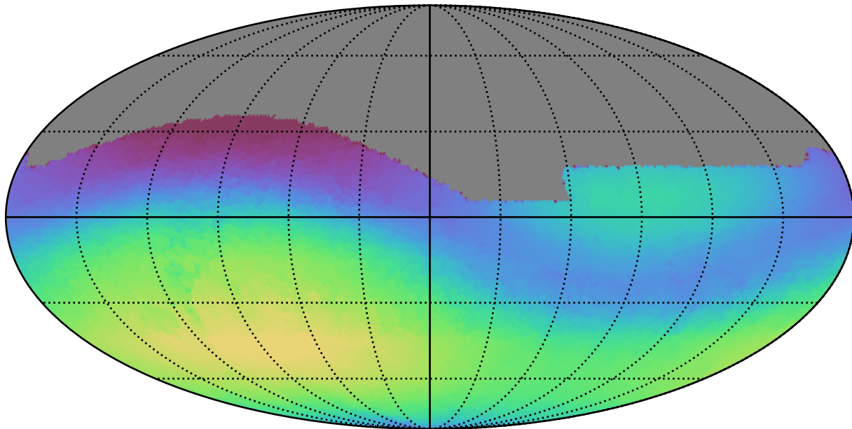
weather_cloudso14v3.4_10yrs All sky g band: Max skyBrightness
