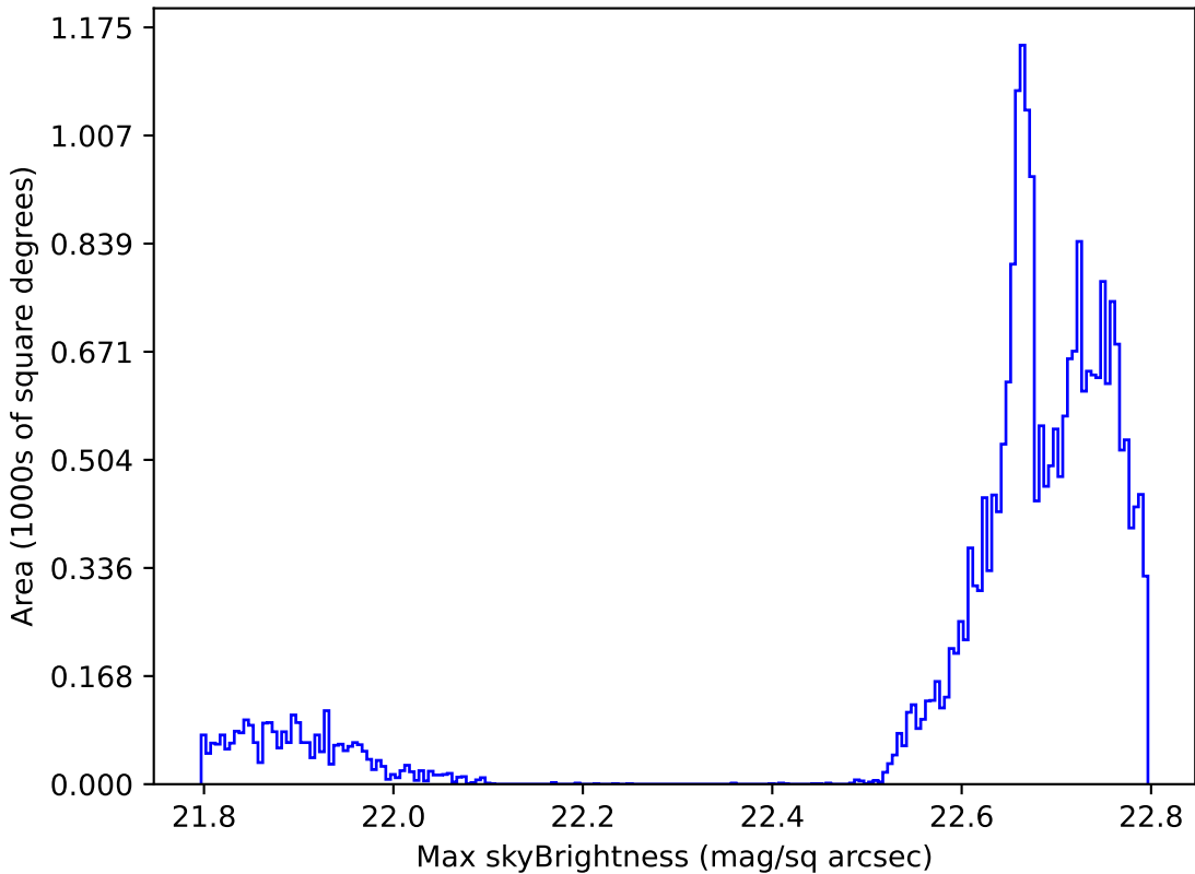
weather_cloudso14v3.4_10yrs All sky all bands: Max skyBrightness
