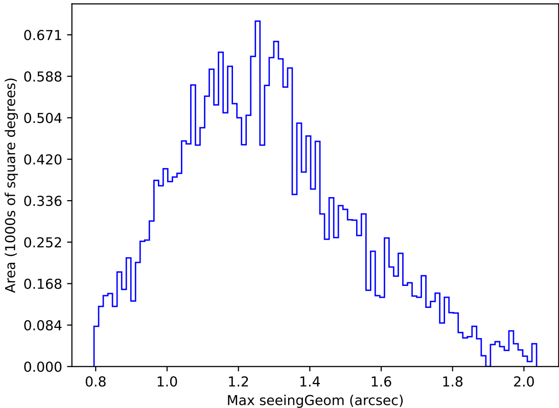
weather_cloudso14v3.4_10yrs Yr 1 g band: Max seeingGeom
