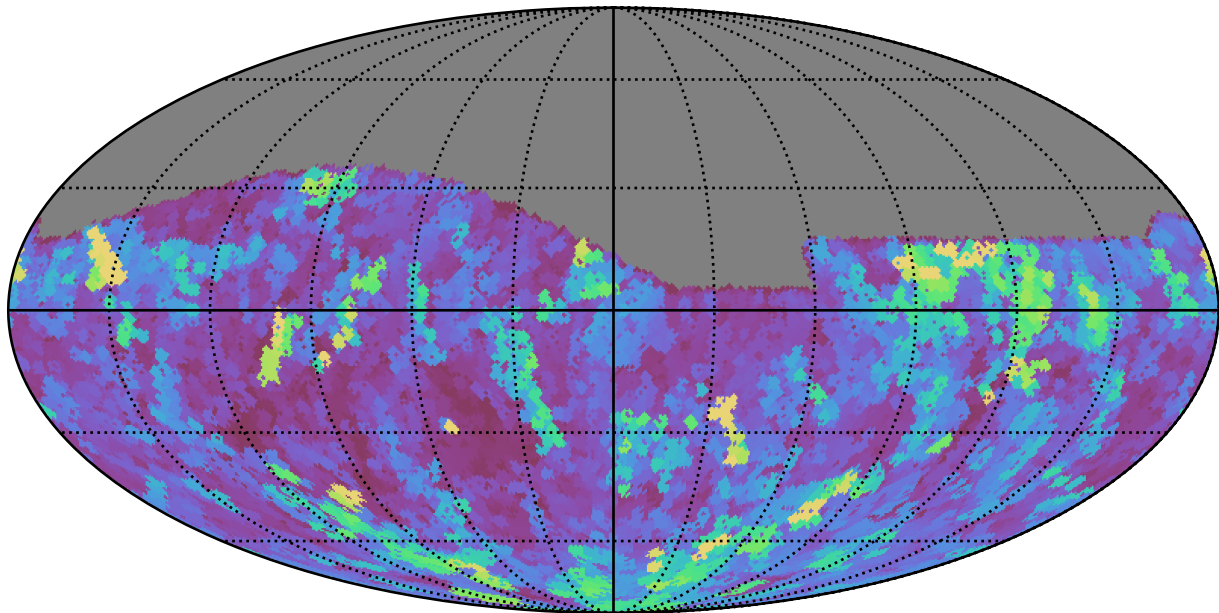
weather_cloudso14v3.4_10yrs Yr 1 all bands: Max seeingGeom
