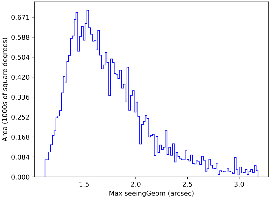
weather_cloudso14v3.4_10yrs Yr 1 all bands: Max seeingGeom
