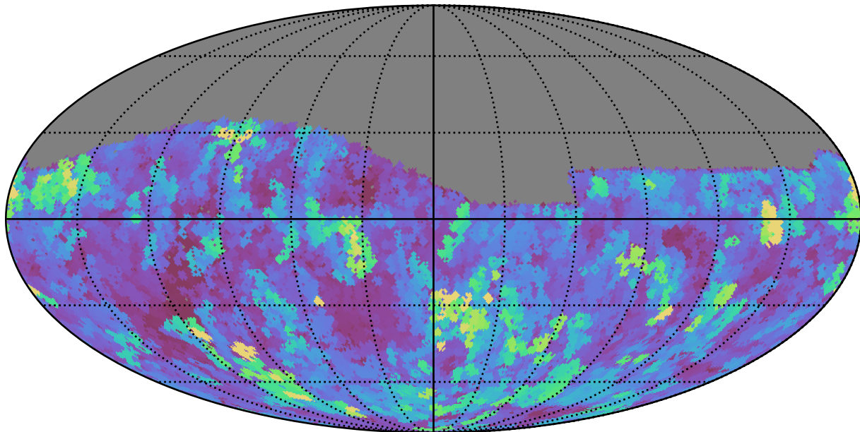
weather_cloudso14v3.4_10yrs Yr 1 z band: Max seeingEff
