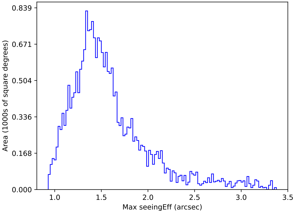
weather_cloudso14v3.4_10yrs Yr 1 u band: Max seeingEff
