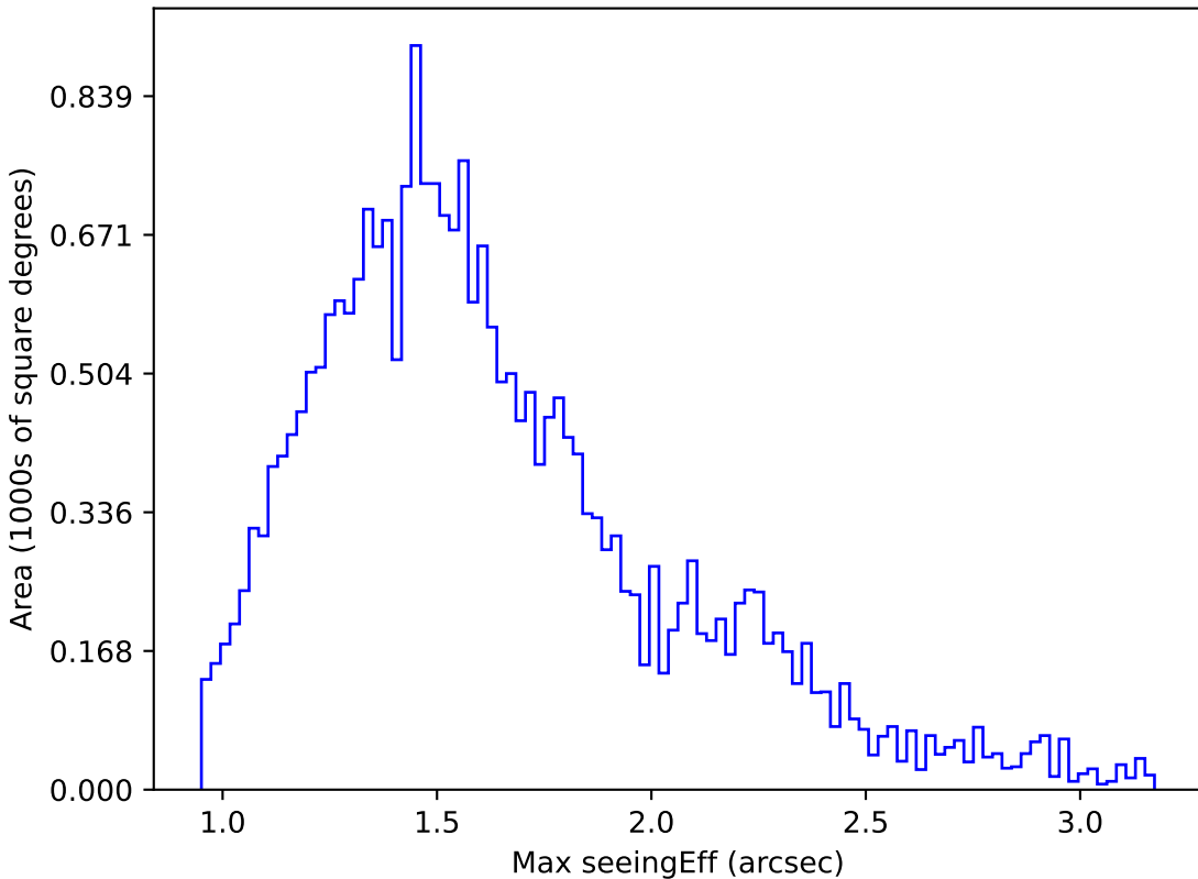
weather_cloudso14v3.4_10yrs Yr 1 r band: Max seeingEff
