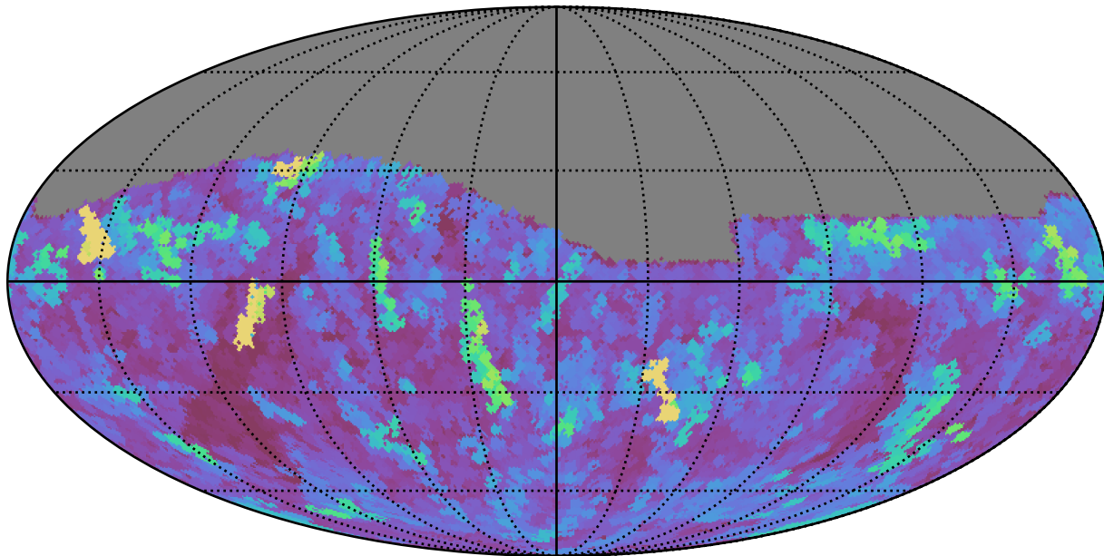
weather_cloudso14v3.4_10yrs Yr 1 i band: Max seeingEff
