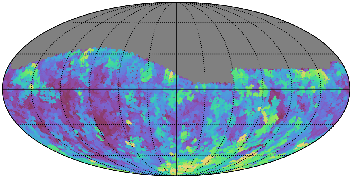
weather_cloudso14v3.4_10yrs Yr 1 g band: Max seeingEff
