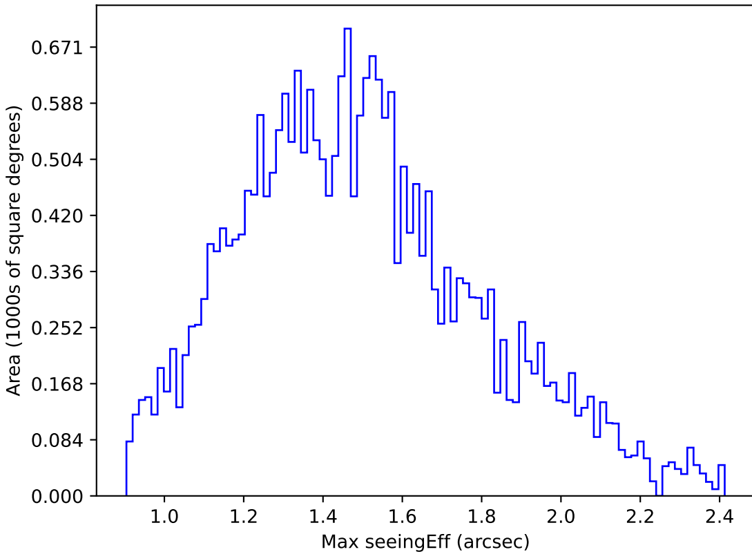
weather_cloudso14v3.4_10yrs Yr 1 g band: Max seeingEff
